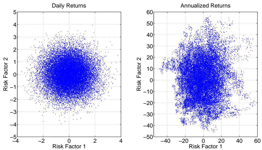
Figure 5: Time series plots of simulated annualized returns (top) and scatter plots of daily (bottom left) and annualized (bottom right) return series
