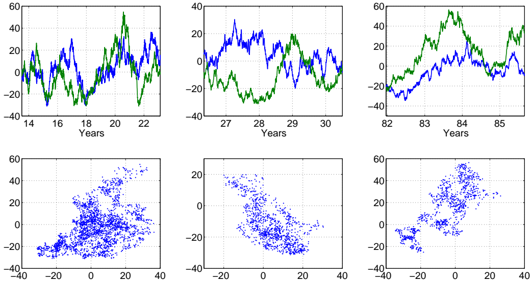
Figure 6: Selected subsets of the annualized return series showing time series plots (top) and corresponding scatter plots (bottom) with sample correlations \hat{\rho} = 0.42 , \hat{\rho} = -0.65 and \hat{\rho} = 0.75 (from left to right)
