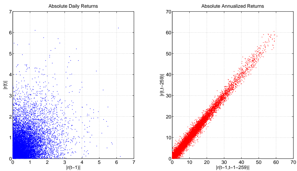
Figure 2: Sample autocorrelations (top) and scatter plots of GARCH-simulated absolute daily (bottom left) and absolute annualized (bottom right) returns
