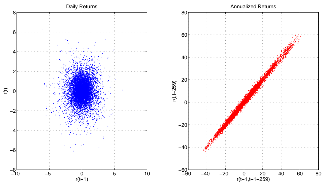
Figure 1: Sample autocorrelations (top) and scatter plots of simulated daily (bottom left) and annualized (bottom right) returns
