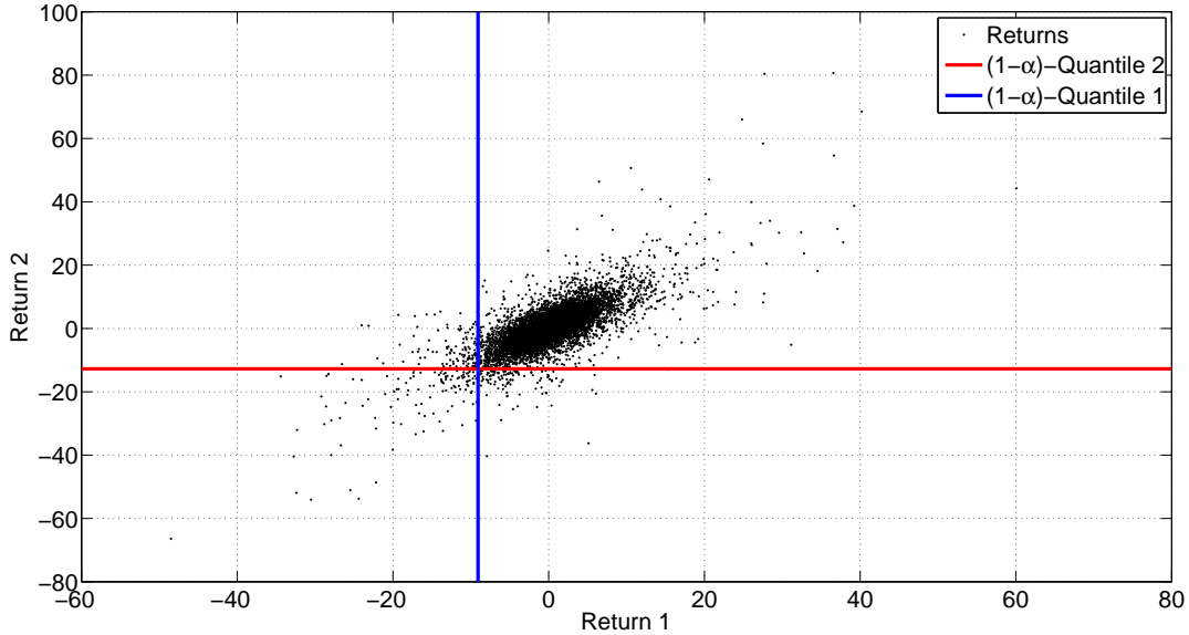
Figure 7: Tail correlation via data-cutting approach
