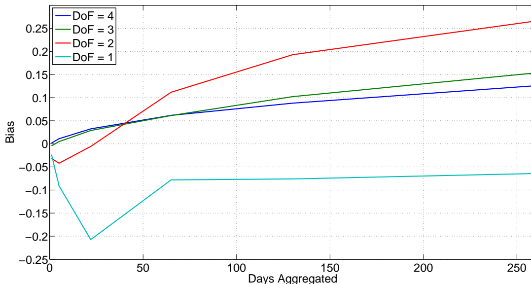
Figure 19: Bias due to rolling–window aggregation for t –distributed daily returns with \rho = 0.0 and different degrees of freedom
